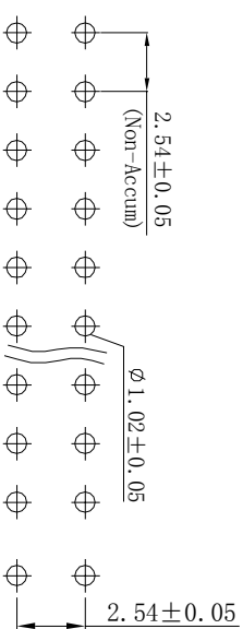
PCB LAYOUT
