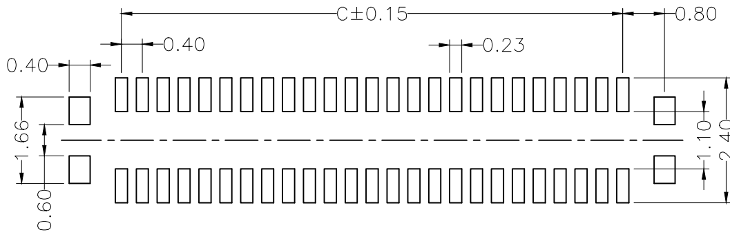
RECOMMENDED PCB LAYOUT CONNECTOR SIDE
